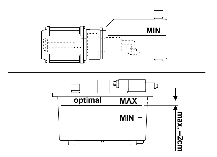
Fig. 8: Oil level
