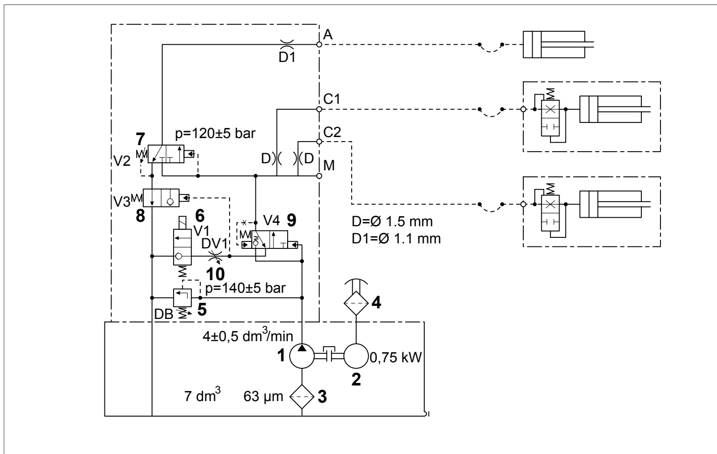
Fig. 5: Hydraulic plan
