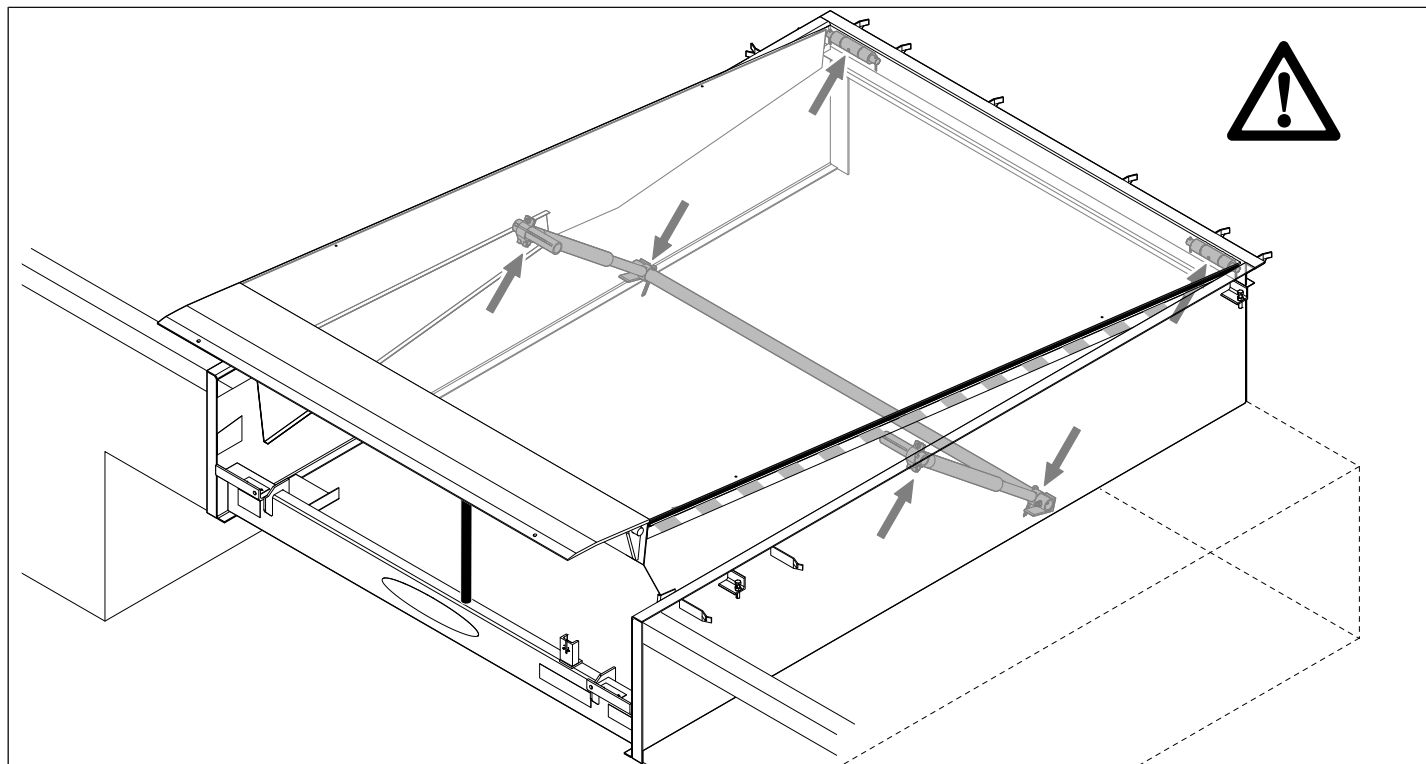
Fig. 7: Lubrication points, illustration may deviate from the product
