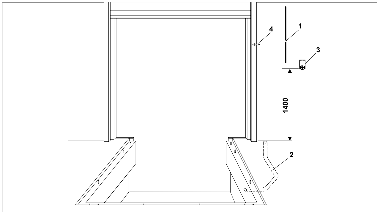
Fig. 6: Exemplary representation for installation situation CZ
